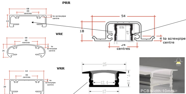
LED Aluminium Extrusion Recessed Profile for LED strip ALU-1706B
