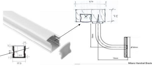
ICL Oneup Aluminium Profile 17mm X 15mm X INT 12.4mm, opal diffuser, end caps and mounting clips c/w Atlas 9.6/m 4000K IP20 LED Tape with CRI 90 and remote NON DIMMING control gear
