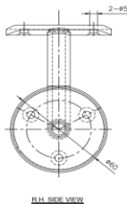
Handrail Brackets with a hollow stem for running electrical cable Enables connection to power for LED light strip (not included)
