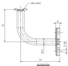
Handrail Brackets with a hollow stem for running electrical cable Enables connection to power for LED light strip (not included)
